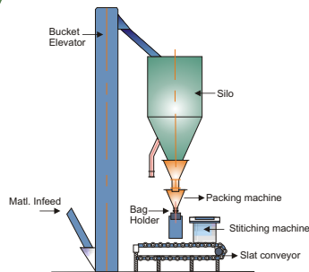
Electronic Stationary-Packer
